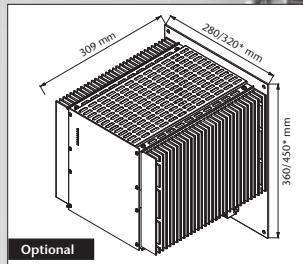
Optional Wall mount approx. 19 kg/ *) 22 kg *) applicable to models >= 150 A input or output current
