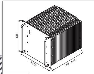
Standard Eurocassette (pluggable module for 19" sub-rack)
