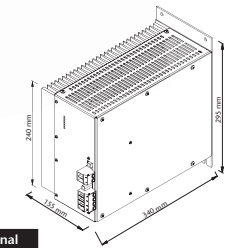
Optional Chassis mount (available for currents up to 60Amps) approx. 10.0 kg
